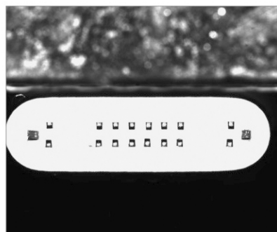
CST-RS7390-B USB针脚检测
