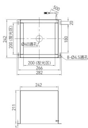
CST-LB-242-242-211 1
