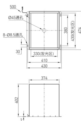
CST-LB-474-430-402 3
