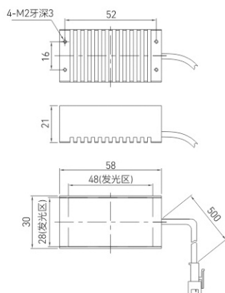
CST-POH4828
