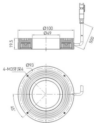
CST-POR10090
