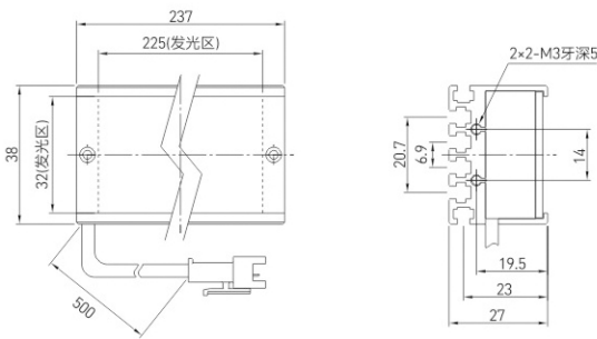
CST-POH4828
