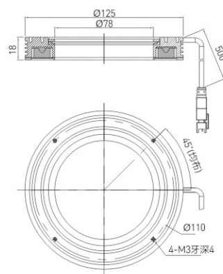
CST-POR12590
