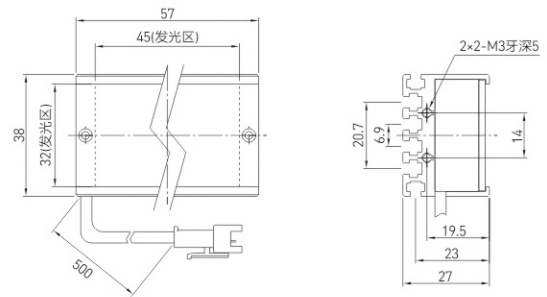
CST-2POB14738
