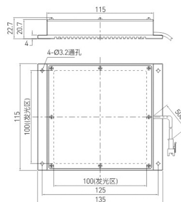
CST-POH100100
