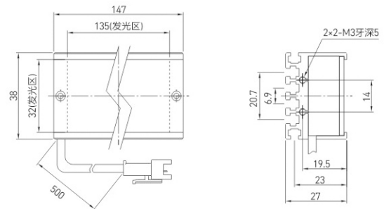
CST-2POB32738
