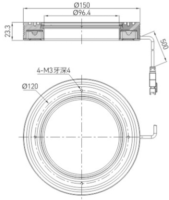
CST-POB10228
