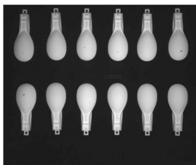
CST-2POB327338-W 勺子脏污检测
